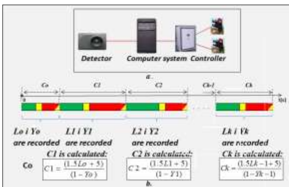
Fig.1. System elements and cycle calculation
