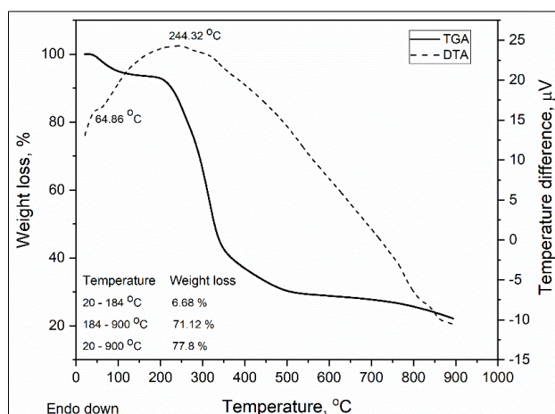
Figure 3. DTA-TGA analysis of bean shells
