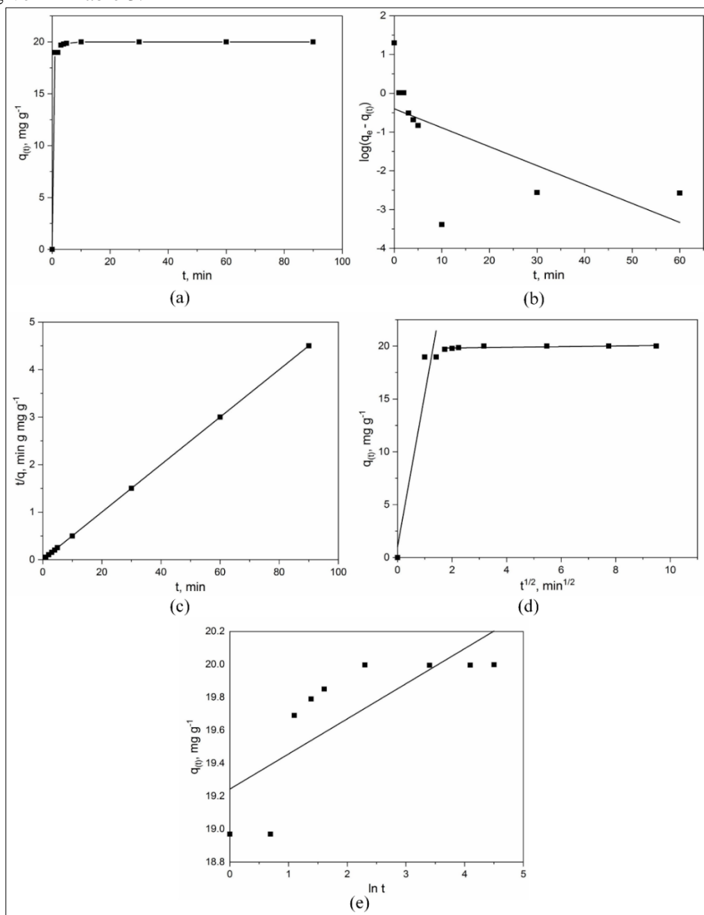
Figure 8. Change in the adsorption capacity with time (a); pseudo-first order kinetic model (b); pseudo-second order kinetic model (c); intraparticle diffusion kinetic model (d); Elovich kinetic model (e)
