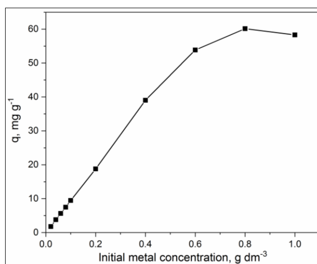
Figure 7. The influence of the initial concentration of lead ions on the adsorption capacity
