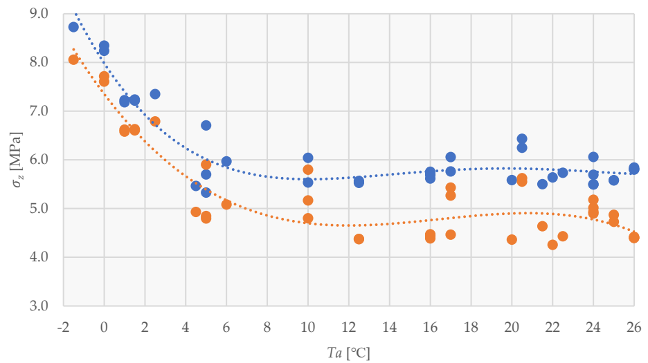
Figure 26. Extreme values of \sigma_z [MPa] as a function of ambient temperatures T_a [°C] (blue—monolith length 20.0 m; orange—monolith length 15.0 m).
