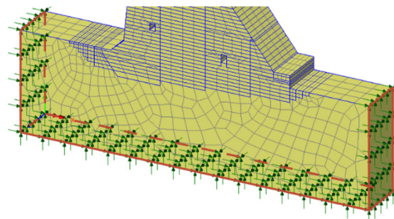
Figure 6. The boundary condition for conducting stress analysis.
