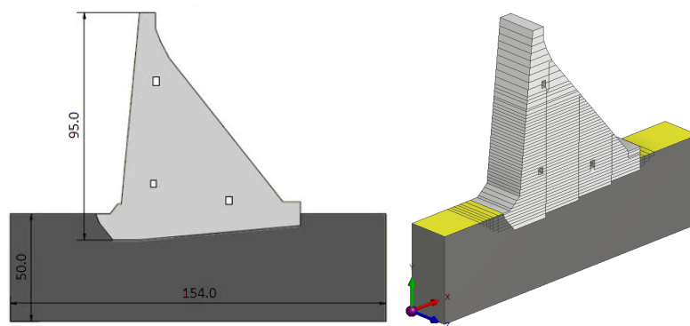
Figure 3. (Left): Characteristic cross-section; (right): 3D model of the monolith with 78 blocks and the surrounding rock mass for thermal stress analysis.
