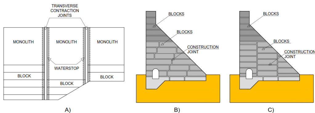
Figure 1. Waterstops, blocks, and joints of a concrete gravity dam: (A) waterstops between adjacent monoliths; (B) combination of long blocks and staggered joints; (C) combination of long blocks and vertical joints.
