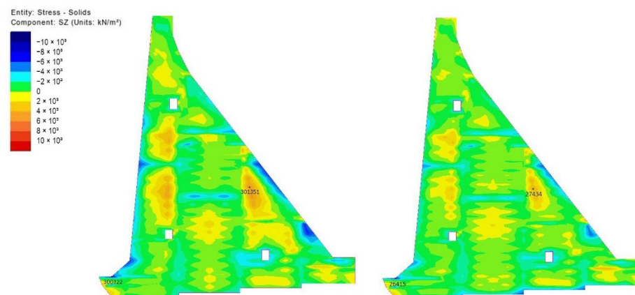
Figure 23. Stresses \sigma_z in the mid-plane of the monolith 20 m long (left) and 15 m long (right) for the 1804th day (25th of September of the sixth year); extremums: nodes 301,351 and 27,434.
