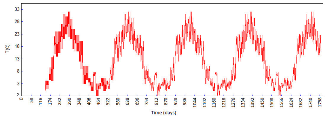
Figure 10. Concrete temperature (°C) in node 2853 (downstream face).
