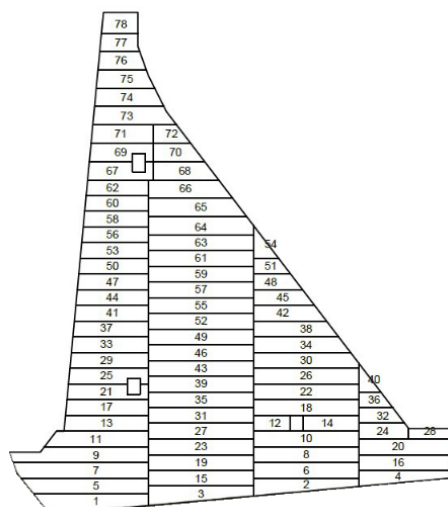
Figure 4. Concrete blocks in the gravity dam (numbers coincide with the sequence of pouring).
