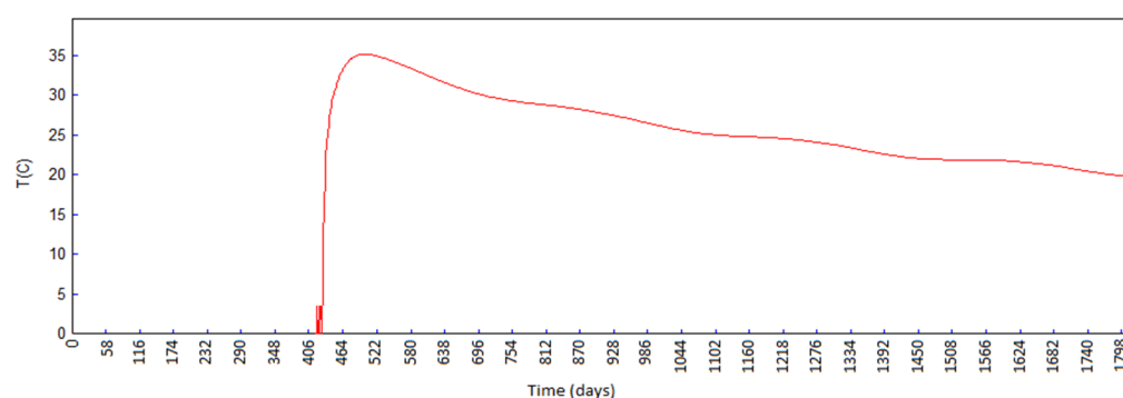
Figure 11. Concrete temperature (°C) in node 3016 (middle of the monolith).
