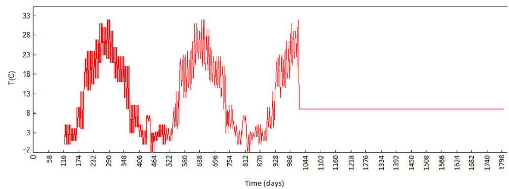
Figure 9. Concrete temperature (°C) in node 2787 (upstream face).
