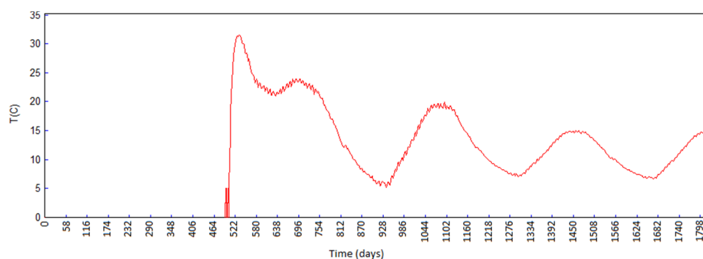
Figure 12. Concrete temperature (°C) in node 3184 (zone of the dam's crest).
