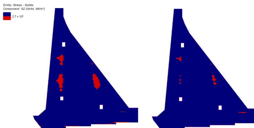
Figure 31. Zones in which the concrete tensile resistance is exceeded (red) in the mid-plane of the monolith 20 m long (left) and 15 m long (right) for the 1804th day from the beginning of construction (25th of September of the sixth year).
