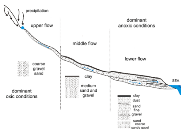
Figure 1 Schematic representation of an alluvial aquifer (Dimkić, 2012)
