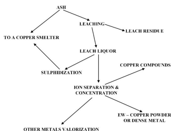
Figure 4. Variants of the ash treatment and metal valorization.
