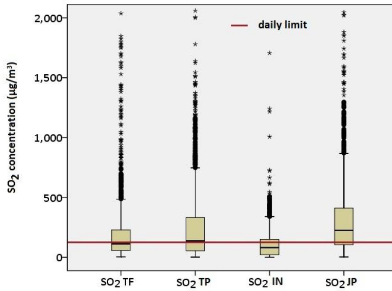
Fig. 2 Box plots of average daily concentrations of SO 2 in Bor in the period 2011-2015
