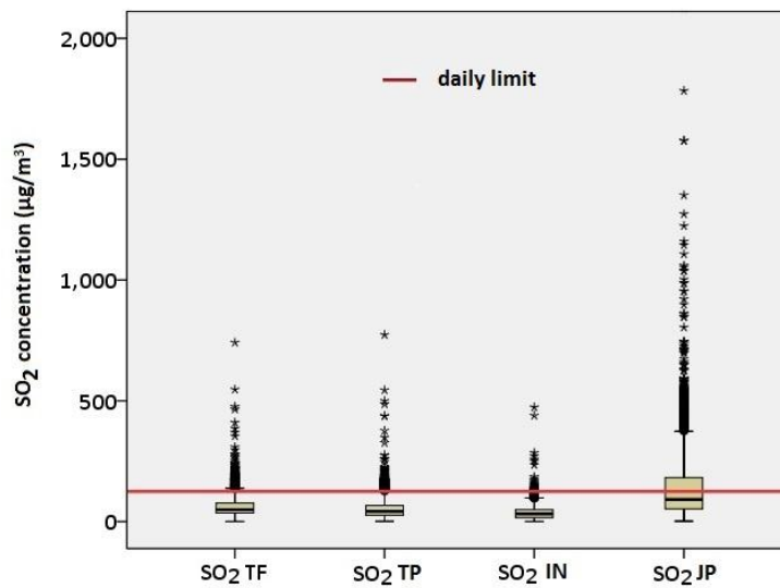
Fig. 3 Box plots of average daily concentrations of SO 2 in Bor in the period 2016-2020
