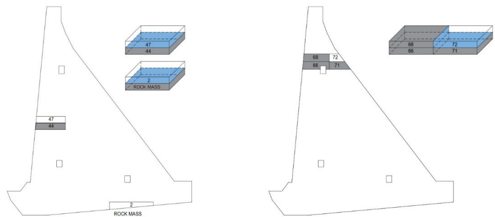
Figure 4. The boundary condition allowing for heat transfer on the contact surfaces of the blocks with the rock mass and the previously cast blocks (the concreting of the block was not shifted).
