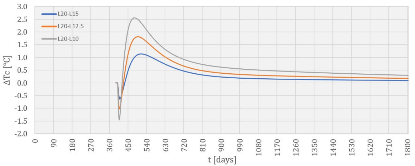
Figure 12. Concrete temperature change ( ^{\circ}\text{C} ) in node 2938, depending on monolith length change.
