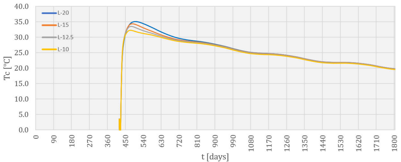
Figure 13. Concrete temperature ( ^{\circ}\text{C} ) in node 3016 (above central zone).
