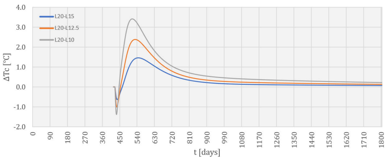
Figure 14. Concrete temperature change ( ^{\circ}\text{C} ) in node 3016, depending on monolith length change.
