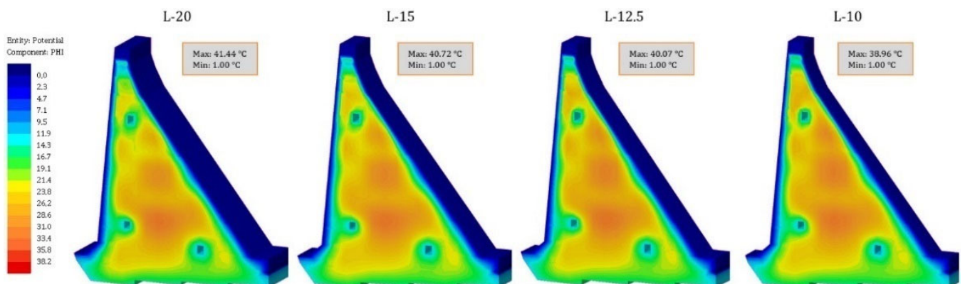
Figure 20. Isometric view of the TF for different monolith lengths (512th day—13 March of the 3rd year).
