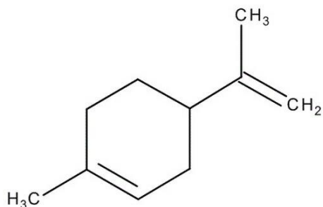
Figure 5. Structure of limonene, the principal component of C. Lawsoniana essential oil
