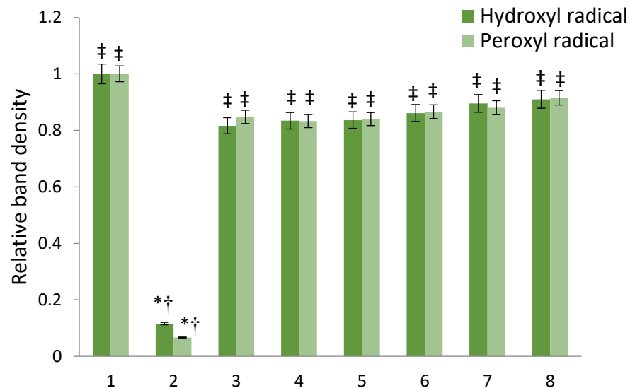
Figure 3. Protective potential of essential oil of Chamaecyparis lawsoniana against hydroxyl and peroxy radicals-induced DNA damage. DNA from salmon sperm (1, negative control), DNA damage control (2, positive control), quercetin (3, 0.01%, standard), essential oil in concentrations of 3, 1.5, 0.75, 0.38, and 0.19% (4, 5, 6, 7, and 8).
