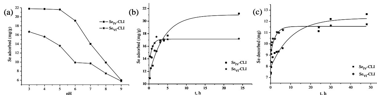
Figure 2. (a) Adsorption of Se(IV) and Se(VI) on Fe-CLI as a function of pH; (b) adsorbed amount of Se(IV) and Se(VI) on the Fe-CLI in time, and (c) desorbed amount of selenium from Se IV -CLI and Se VI -CLI samples in time.
