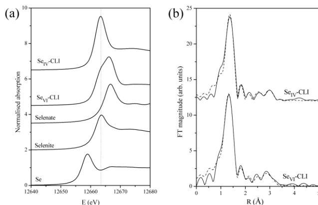
Figure 3. (a) Se K-edge XANES of Se-containing zeolite samples Se IV -CLI and Se VI -CLI together with reference Se compounds (selenite, selenate and elemental Se); (b) Fourier transforms of k 3 -weighted Se K-edge EXAFS spectra of Se IV -CLI and Se VI -CLI samples (experiment: solid line; best fit EXAFS model: dashed line).
