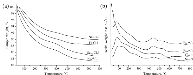
Figure 1. TG (a) and DTG curves (b) of Na-CLI, Fe-CLI, Se IV -CLI and Se VI -CLI. This is explained by interactions of selenite and selenate ions with the Fe(III)-modified surfaces.
