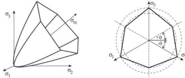
Figure 1. Failure surface of Hoek-Brown material model
